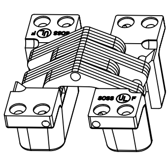
HINGE OPEN 180° ISOMETRIC VIEW
