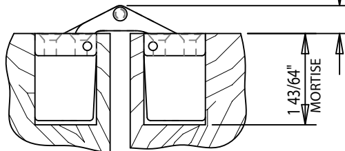
HINGE OPEN 180° TOP VIEW CUT AWAY
