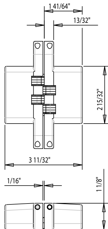
HINGE CLOSED FRONT VIEW CUT AWAY
