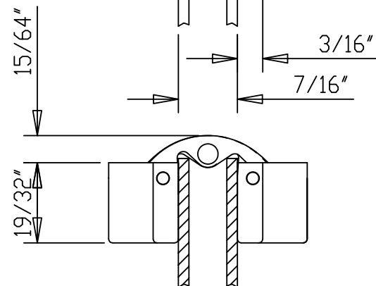
HINGE OPEN 180° TOP VIEW
