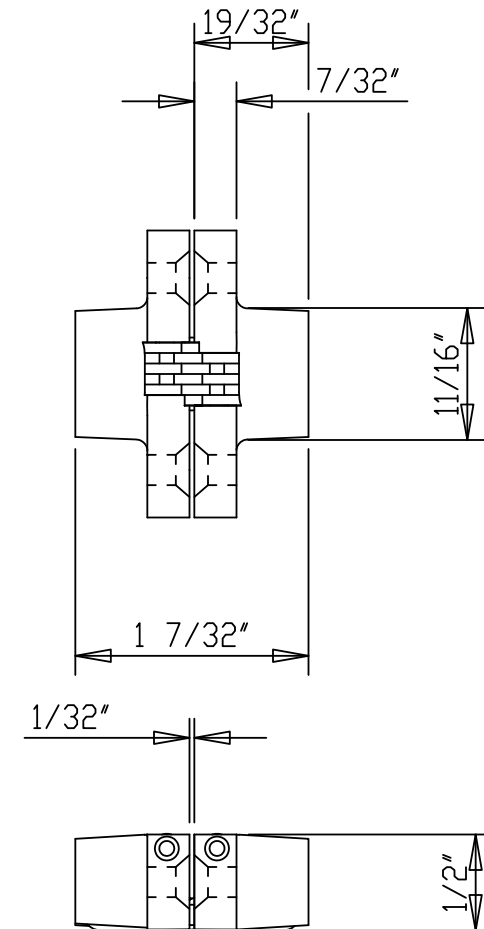
HINGE CLOSED FRONT VIEW CUT AWAY
