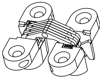
HINGE OPEN 180° ISOMETRIC VIEW
