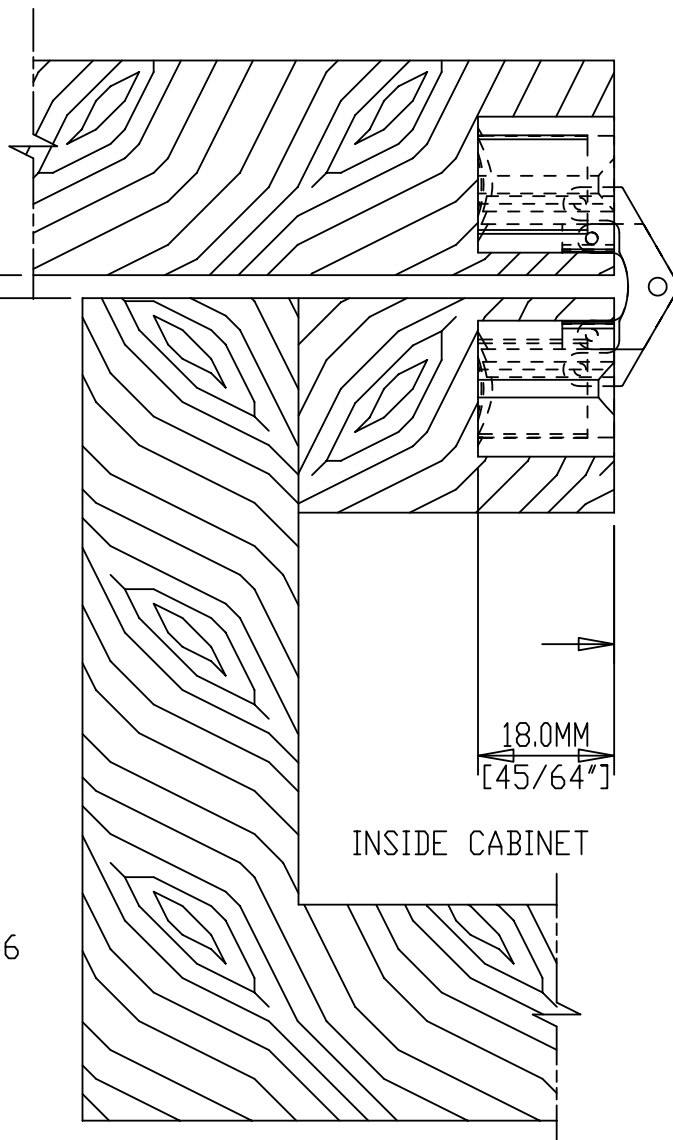
HINGE OPEN 180° SIDE VIEW CUT AWAY
