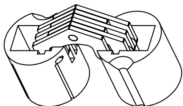
HINGE OPEN 180° ISOMETRIC VIEW
