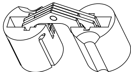
HINGE OPEN 180° ISOMETRIC VIEW
