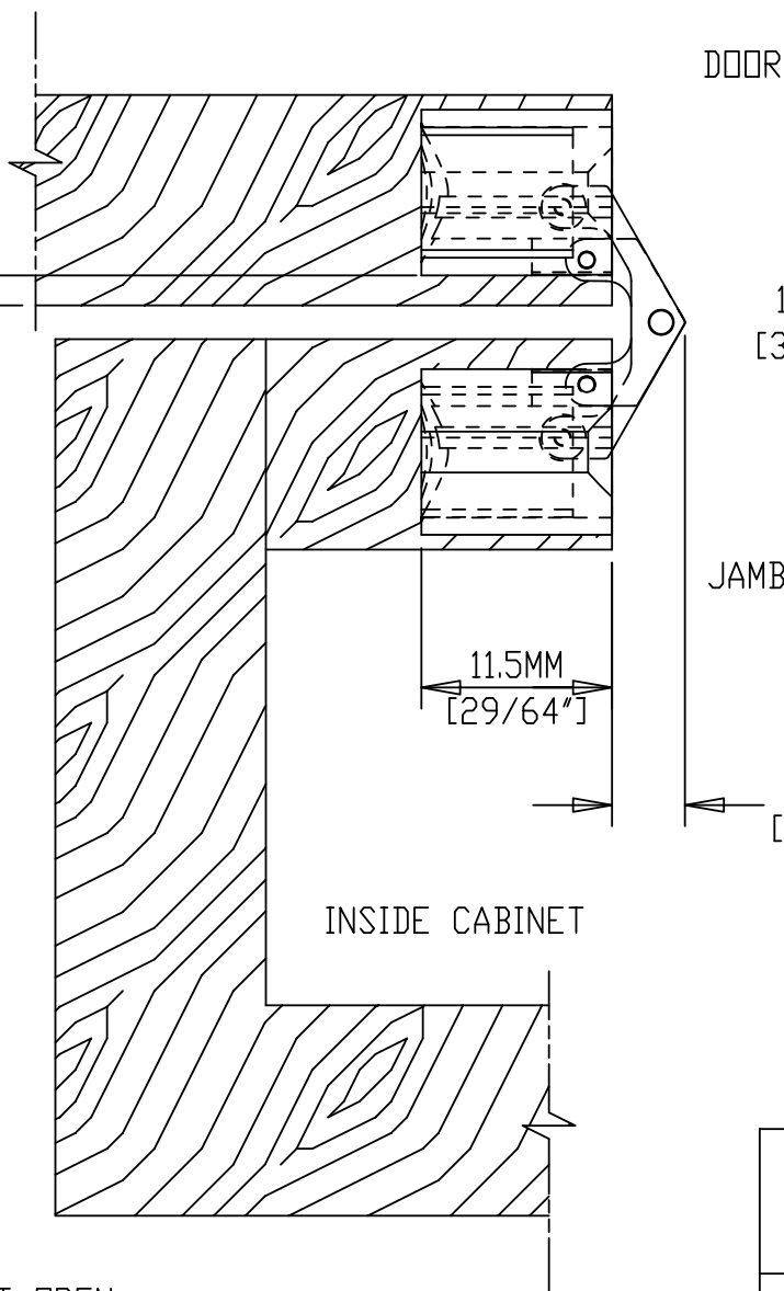
HINGE OPEN 180° SIDE VIEW CUT AWAY
