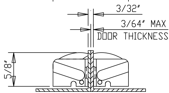
HINGE CLOSED° TOP VIEW
