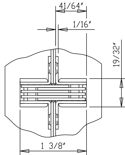
HINGE CLOSED FRONT VIEW
