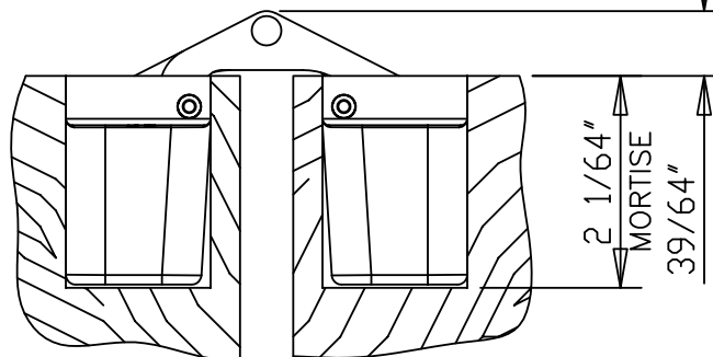
HINGE OPEN 180° TOP VIEW CUT AWAY
