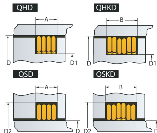
Product Dimensions All dimensions in millimeters unless otherwise specified.
