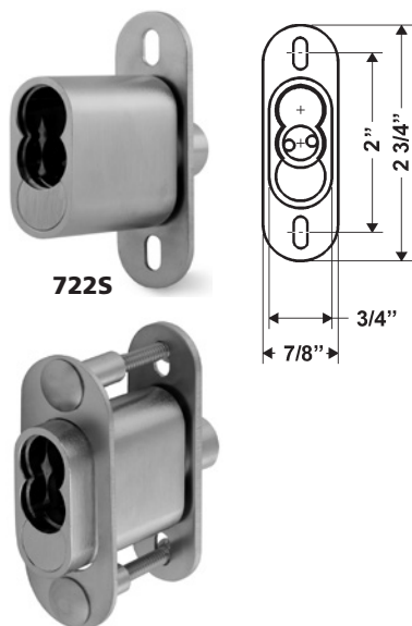
722S-TBM Through-bolt mount
