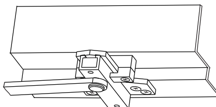
DEEP REVEAL APPLICATION WITH 9500-DRK CLAMP KIT
