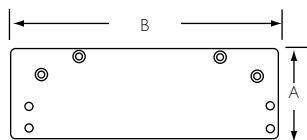
Closer Mounting Plate
