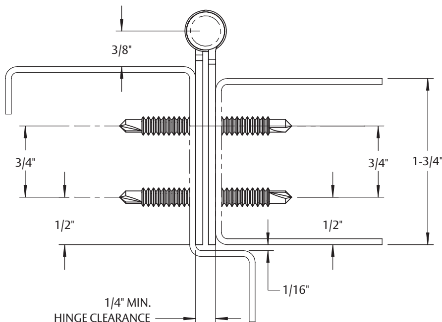
Fig. 2 HINGE PLACEMENT & CLEARANCE TEMPLATE
