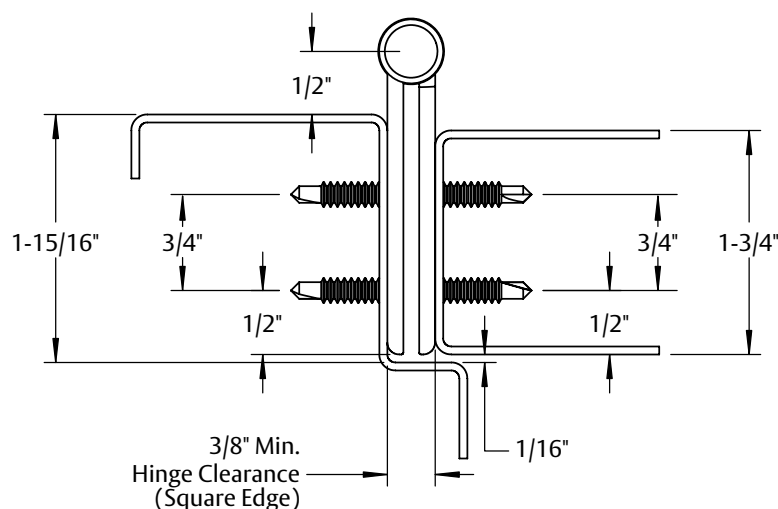
Fig. 2 HINGE PLACEMENT & CLEARANCE TEMPLATE
