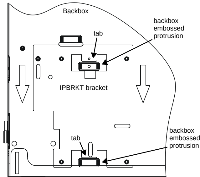
Figure 1 IPBRKT Installation
