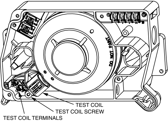
FIGURE 9. SK-DUCT WITH OPTIONAL TEST COIL
