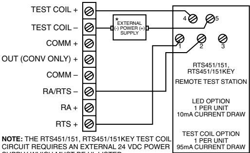
FIGURE 10. WIRING DIAGRAM FROM SK-DUCT TO RTS451/RTS151, RTS451KEY/RTS151KEY:
