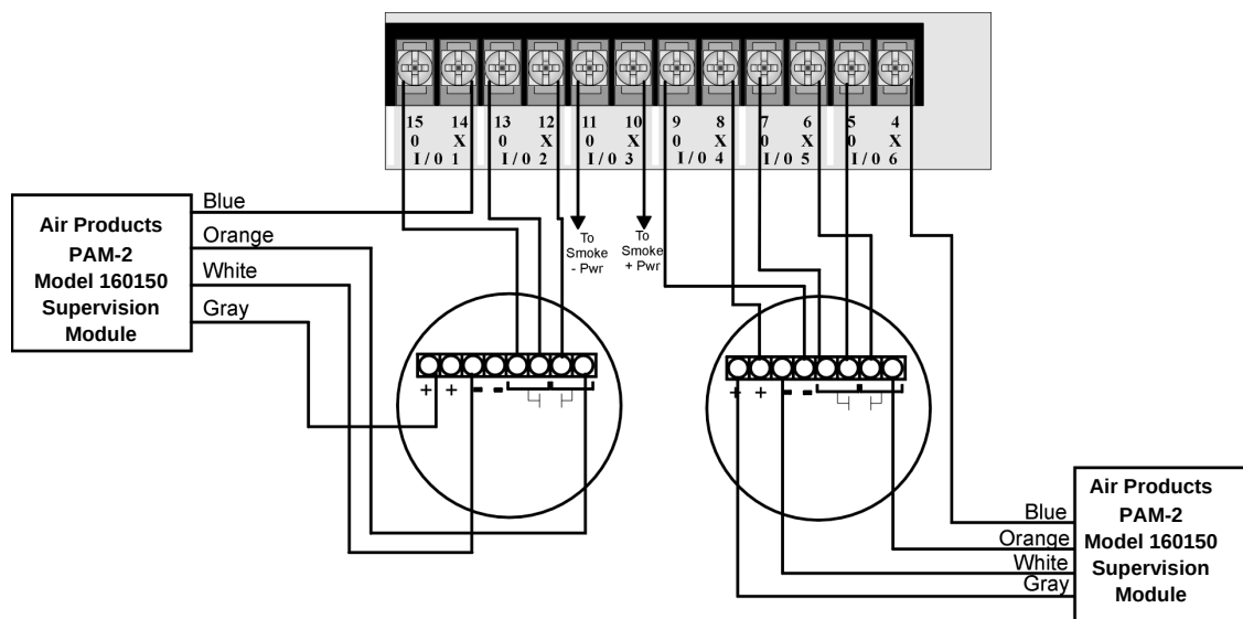
Figure 3-15 Class A 4-Wire Smoke Detector Connections
