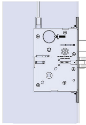
52XX Primary bolt & top deadbolt
