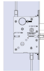
53XX Primary, top & bottom vertical deadbolts
