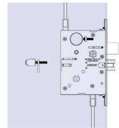
54XX Primary, top & bottom vertical deadbolts, & hinge side stationary deadbolt
