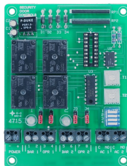
EMC - Exit Device Sequencer Dual Channel Exit Device Sequencer Module
