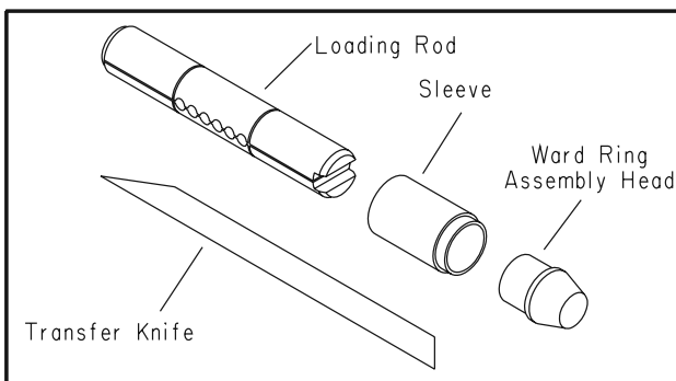
Cylinder Body Loading Tool 40-116
