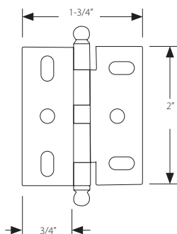
MORTISE BALL TIP
