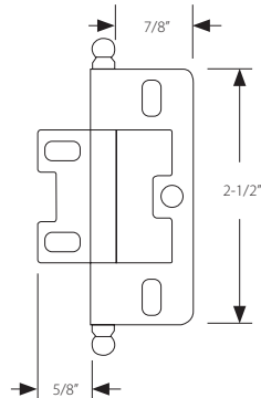
NON-MORTISE BALL TIP
