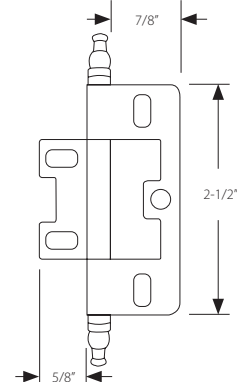
NON-MORTISE MINARET TIP
