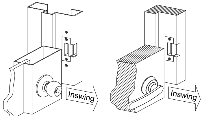
Hollow Metal
