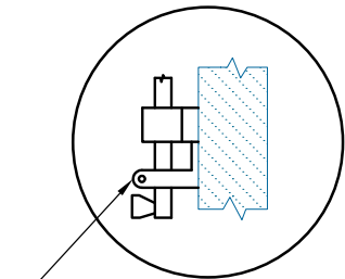
SINGLE LOCK BRACKET FOR PAD LOCK (BOLT SHOWN IN UNLOCKED POSITION)
