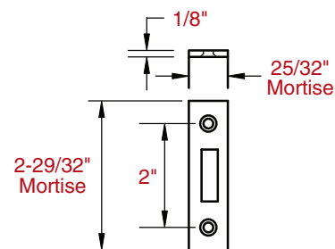
MORTISE STRIKE
