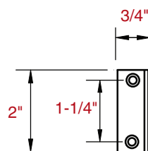
L STRIKE
