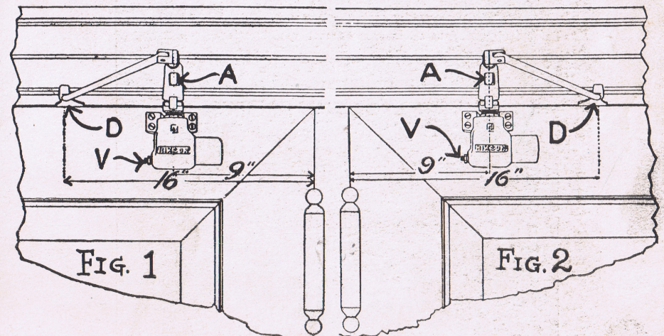
Showing Position of Check When Hinges are on Left-Hand Side.
