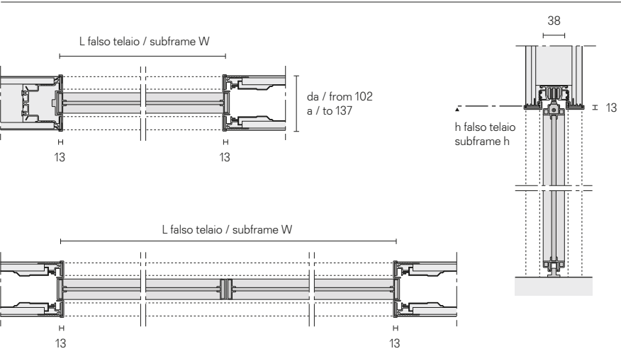
A. Luce netta falso telaio Measure of the subframe C. Luce netta passaggio Dimensions of the opening
