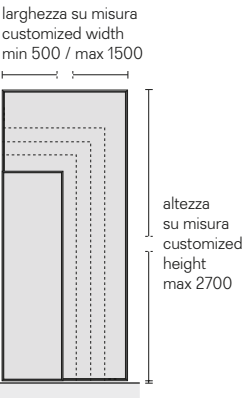
Dimensioni pannelli porta Door panel dimensions
