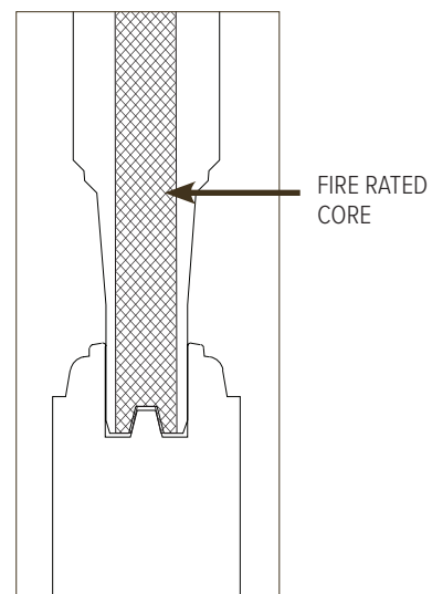
Panel Profile
