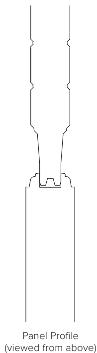
F7304 1-7/16" Beaded V-Groove Double Hip Raised Panel Wide Layout, Ovolo Sticking
