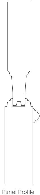
SM7282RM 1-7/16" Double Hip Raised Panel Wide Layout Raised Moulding, 1 Side Ovolo Sticking 3/0 x 6/8 3/0 x 7/0
