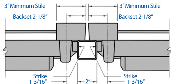
Rim Devices with S458 Strikes and Mullion
