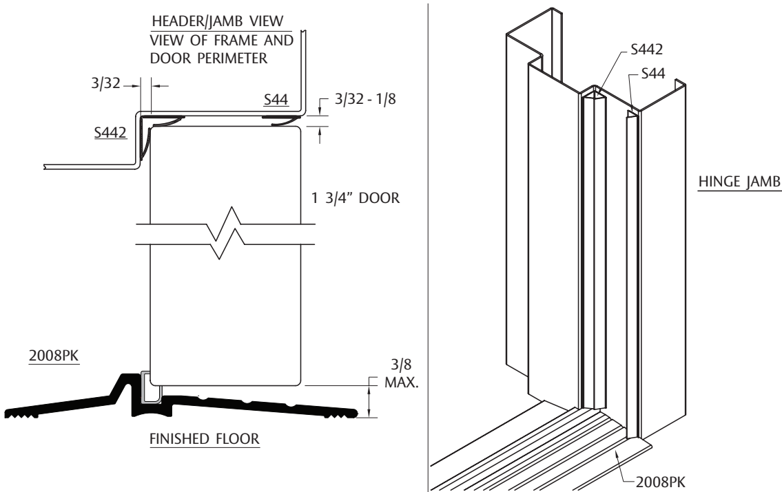
System Detail of an Acoustical Seal Set for Door & Frame
