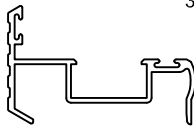
SLIMLINE STYLE 3493, 3494
