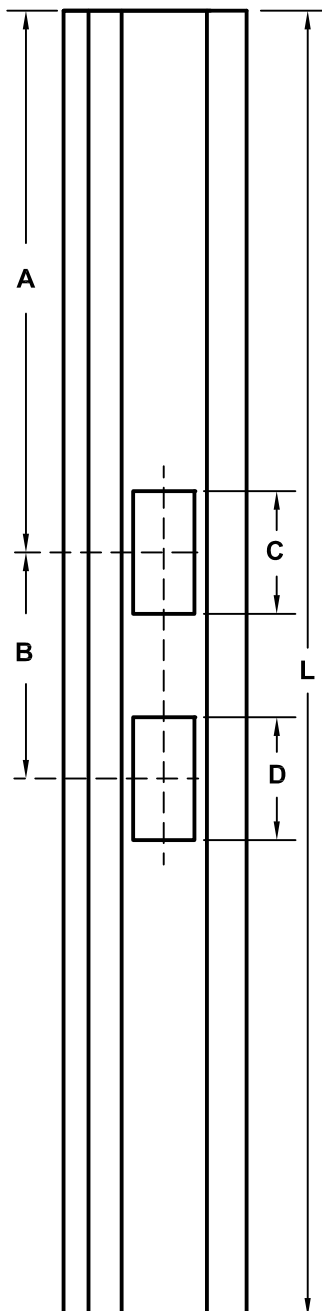
SLIMLINE STYLE 3493, 3494
