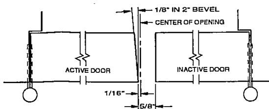
FIG 1 PREPARATION FOR SLIMLINE AND COLONIAL ASTRAGALS
