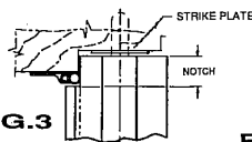
FIG.3 MORTISE AND SLIMLINE STYLES WITH JAMB-UP TYPE WEATHER SEALS (PEMKO 303AV SHOWN)
