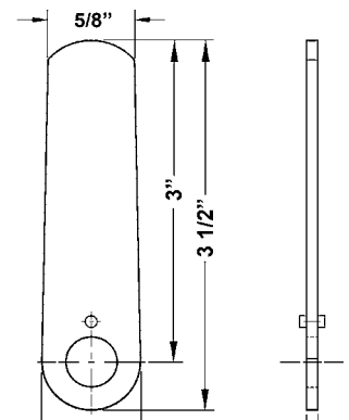
DCNP-100-LC long 3" straight cam
