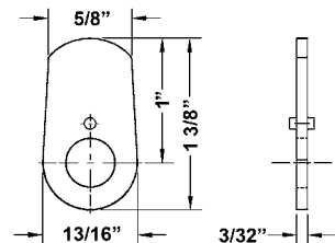
DCNP-HD-1 short cam
