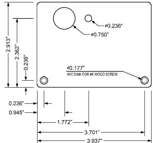
DCP-SP1 - Padlock bumper plate
