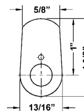
DCNP-100-SC3 1-1/2" heavy duty straight cam
