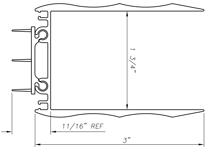
99TA DOOR SHOE PROFILE VIEW
