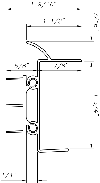
319ET DOOR SHOE PROFILE VIEW
