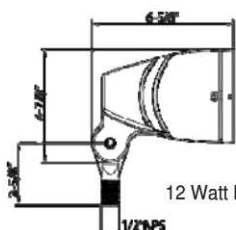
30 Watt Bullet
