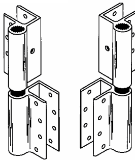
8" HINGE SETS SPECIFY DOOR THICKNESS, PILASTER THICKNESS AND DOOR SWING ADD CENTER HINGE FOR DOORS WIDER THAN 32"
