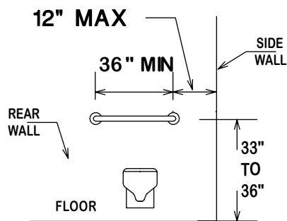
STANDARD STALL REAR WALL
