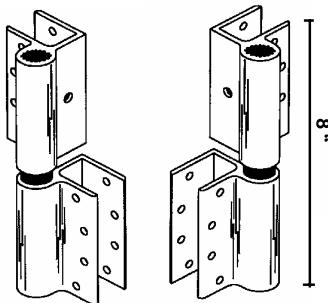
8" HINGE SETS SPECIFY DOOR THICKNESS, PILASTER THICKNESS AND DOOR SWING ADD CENTER HINGE FOR DOORS WIDER THAN 32" SS-4850-8"
