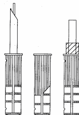
BUMPER-KEEPER OUTSWING CC-2200
