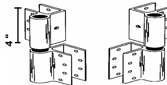
4" HINGE SETS SPECIFY DOOR THICKNESS, PILASTER THICKNESS AND DOOR SWING ADD CENTER HINGE FOR DOORS WIDER THAN 32" SS-4850-4"
