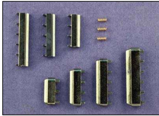
Figure 47 – Medeco Sidebars
