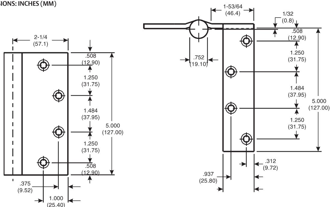
Center &amp; bottom hinge detail
