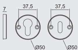
Historia To. paia Bocchette FC/Yale Historia To. pair key hole PK/Yale
