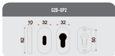
TP.Ov Paia Bocchette FC/Yale TP.Ov pair key hole PK/Yale
