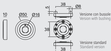
Artax Inox paia rosette Artax Stainless pair roses
