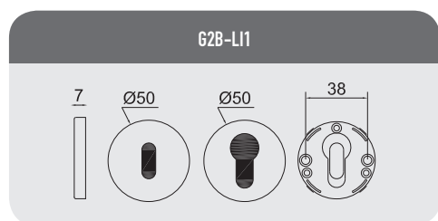
Linz Paia Bocchette FC/Yale Linz pair key hole PK/Yale
