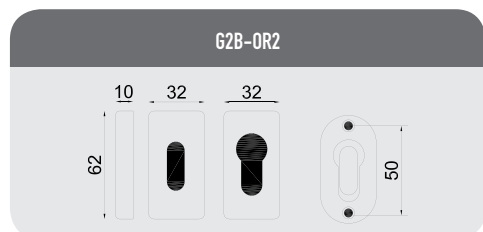
TP.Rt Paia Bocchette FC/Yale TP.Rt pair key hole PK/Yale
