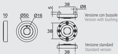
Artax paia rosette Artax pair roses
