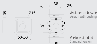
Qbe paia rosette Qbe pair roses
