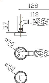
cod. GCW-BAG Maniglia con rosetta/bocchetta Gaia Lever on Gaia rose and key hole
