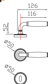
cod. eb. GSB-BAG/pal. GSP-BAG Maniglia con rosetta/bocchetta Gaia Lever on Gaia rose and key hole
