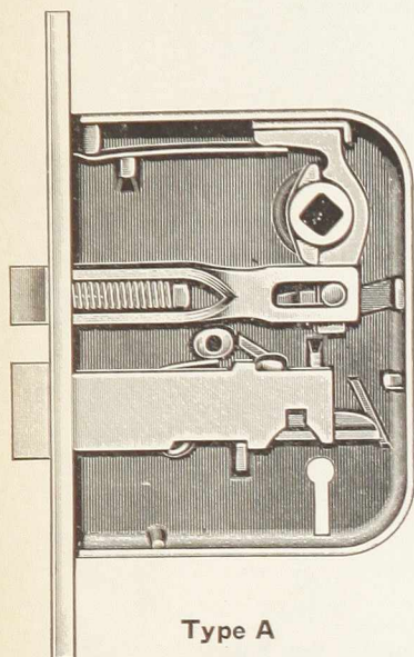
Type A Single Compression Spring
