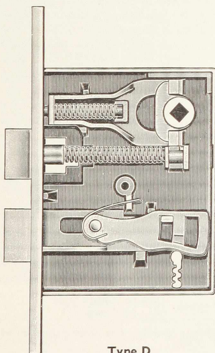
Type D Double Compression Spring
