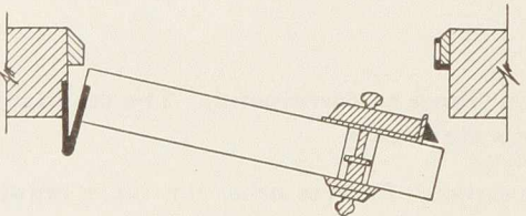
Left Hand Reverse Bevel Lock
