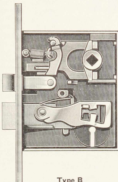
Type B Extension Easy Spring
