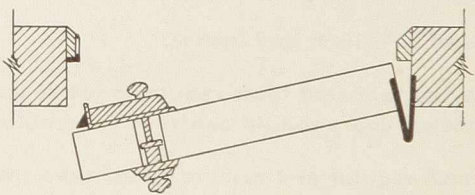
Right Hand Reverse Bevel Lock
