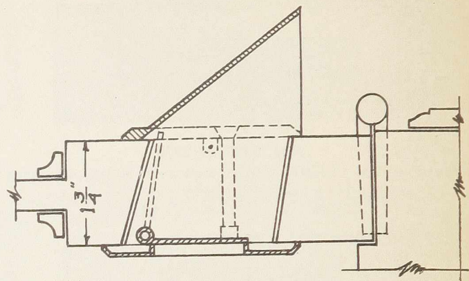
Cross section showing No. JA 275 applied to 1\frac{3}{4} in. Hollow Metal Door in vertical position
