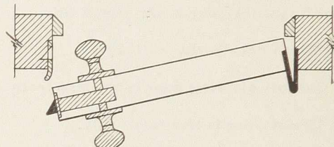
Right Hand Reverse Bevel Lock
