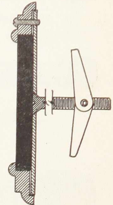
Cross section, showing toggle bolt for fastening
