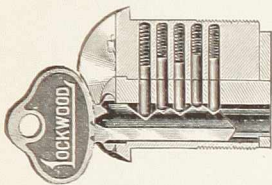
Section showing No. 951 Cylinder
