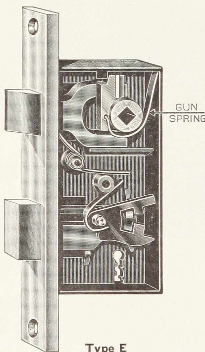
Type E Gun Spring
