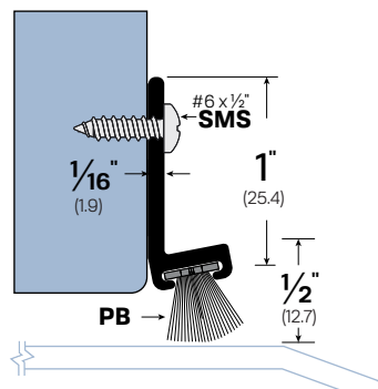
OPTIONAL THRESHOLD OR FINISHED FLOOR
