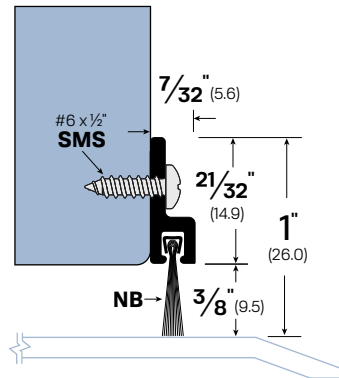
OPTIONAL THRESHOLD OR FINISHED FLOOR
