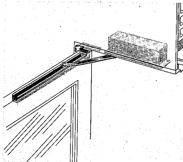
Phantom drawing shows the LCN series 200 OP closer as used with doors hung on offset pivots, a way of clearing certain types of jamb. Door may be of wood, metal or glass having top member at least 1\frac{3}{4} " thick.
