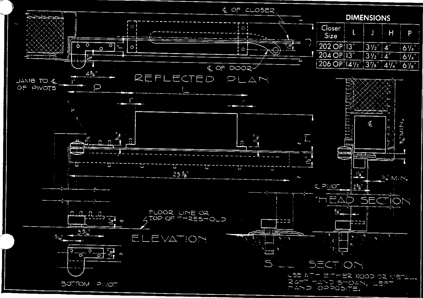
Phantom drawing shows the LCN series 200 OP closer as used with doors hung on offset pivots, a way of clearing certain types of jamb. Door may be of wood, metal or glass having top member at least 1\frac{3}{4} " thick.
