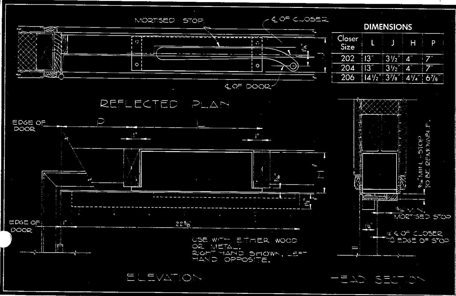
Phantom drawing shows LCN series 200 closer, designed for doors hung on butts. It is entirely independent of the door hanging. Door and/or frame may be wood or metal; if metal, preparation is done by fabricator.
