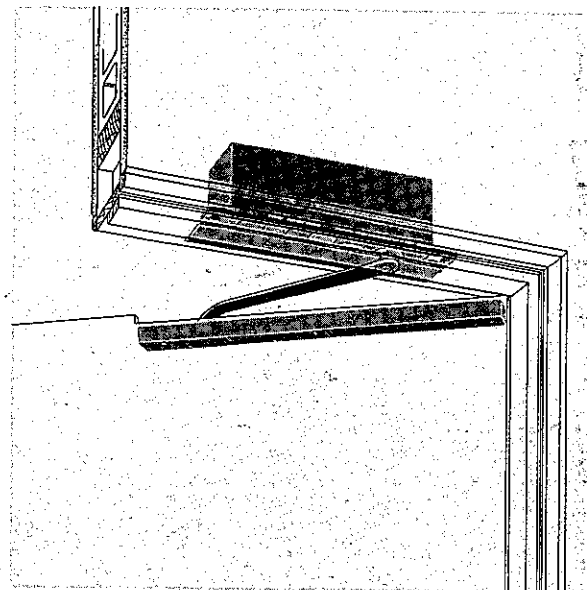
Phantom drawing shows LCN series 200 closer, designed for doors hung on butts. It is entirely independent of the door hanging. Door and/or frame may be wood or metal; if metal, preparation is done by fabricator.
