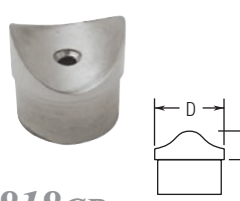
818CP Coped Perpendicular Collar
