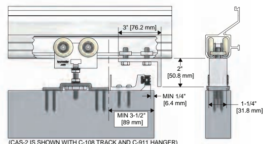
(CAS-2 IS SHOWN WITH C-108 TRACK AND C-911 HANGER)
