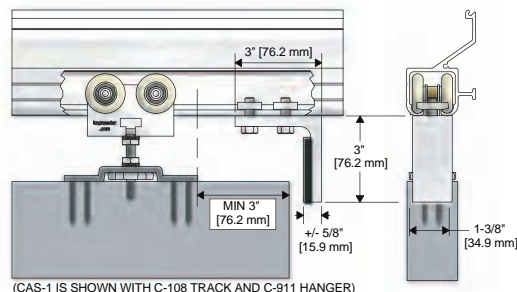
(CAS-1 IS SHOWN WITH C-108 TRACK AND C-911 HANGER)
