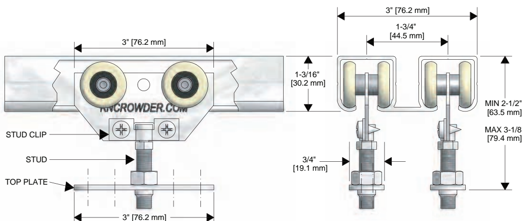
C-304 CONCEALED TYPE HANGER
