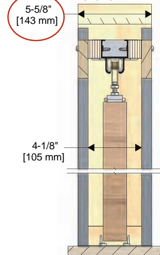
2 X 6 WALL CONSTRUCTION POCKET DOOR KIT SECTION VIEW
