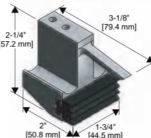
(CDC-911 IS SHOWN WITH C-104 TRACK AND C-911 HANGER)
