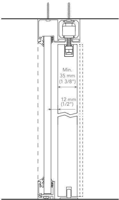
EXPOSED / VISTO
