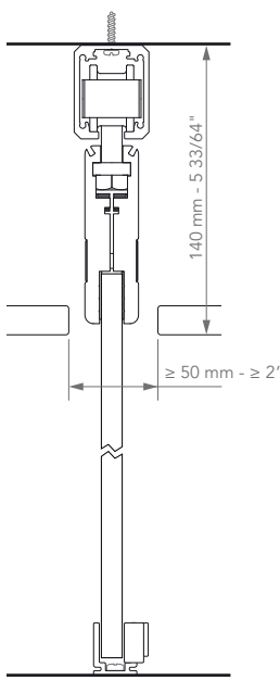
RECESSED / EMPOTRADO
