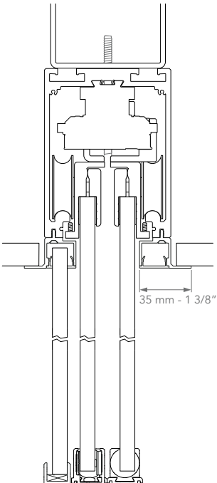
RECESSED / EMPOTRADO
