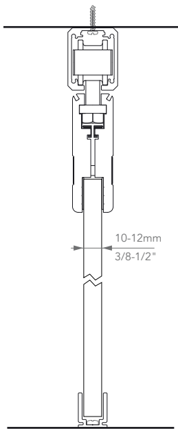
EXPOSED / VISTO
