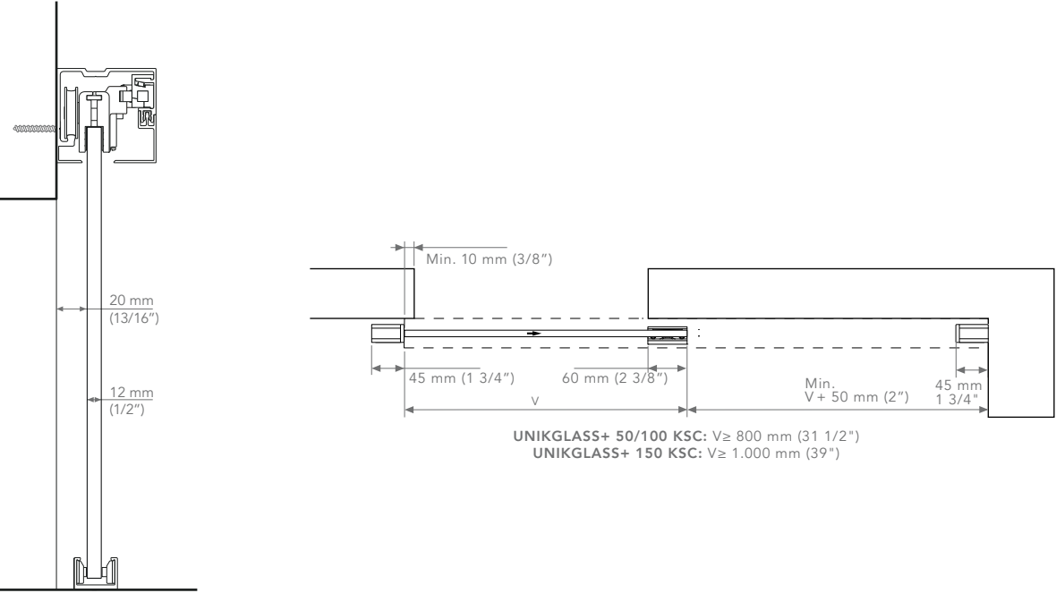
EXPOSED / VISTO
