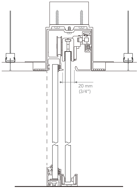
RECESSED / EMPOTRADO
