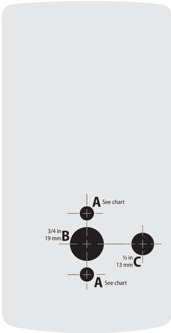
Wall Mount System Escutcheon Footprint (Looking at wall from outside)
